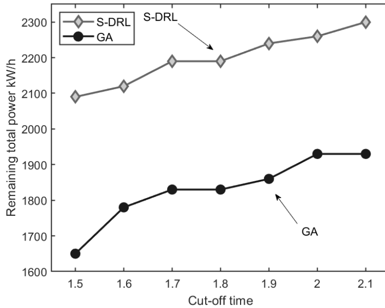
Figure3. The effect of the cut-off time on the total remaining power
