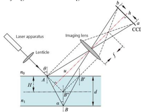
FIGURE 1. Single layer glass physical structure [8]
