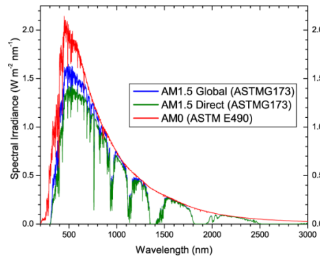
FIGURE 3. AM1.5G standard solar spectrum [9]
