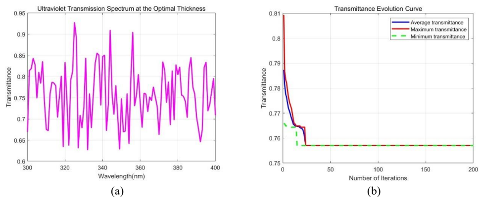
FIGURE 11. UV shielding effect of result 3. (a) Under the optimal thickness combination calculated by traditional genetic algorithm, the transmittance of different wavelengths of ultraviolet light, (b) The variation of ultraviolet transmittance with increasing iteration times (photo/picture credit: original).
