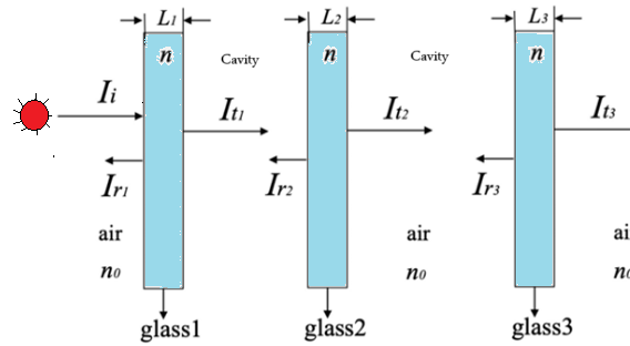
FIGURE 2. Multilayer glass structure (photo/picture credit: original).
