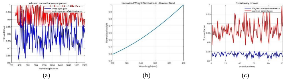
FIGURE 7. Comparison of transmission performance of result 4. (a) Quantum genetic algorithm calculates the transmittance of multi-layer glass and single-layer glass with equal thickness at different wavelengths under optimal thickness, (b) The weight of
