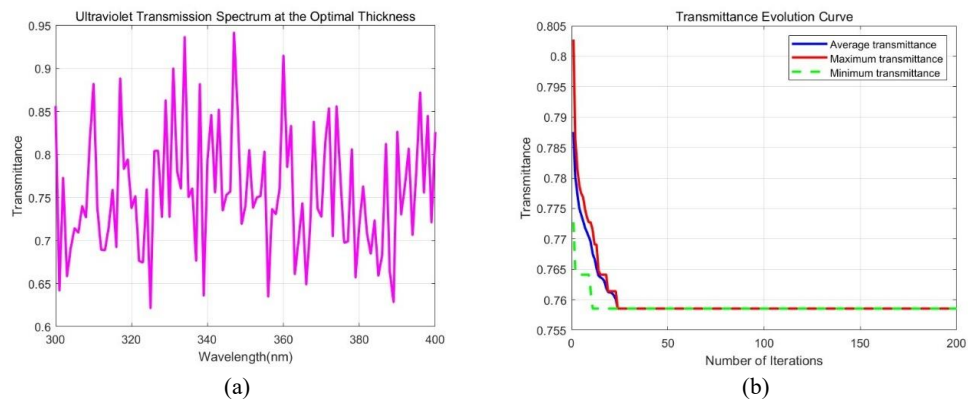
FIGURE 10. UV shielding effect of result 2. (a) Under the optimal thickness combination calculated by traditional genetic algorithm, the transmittance of different wavelengths of ultraviolet light, (b) The variation of ultraviolet transmittance with increasing iteration times (photo/picture credit: original).
