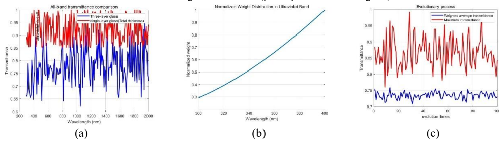
FIGURE 5. Comparison of transmission performance of result 2. (a) Quantum genetic algorithm calculates the transmittance of multi-layer glass and single-layer glass with equal thickness at different wavelengths under optimal thickness, (b) The weight of ultraviolet rays at different wavelengths, and (c) The variation curve of ultraviolet transmittance with increasing iteration times (photo/picture credit: original).
