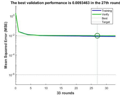
FIGURE 3. Neural network convergence curve (photo/picture credit: original).
