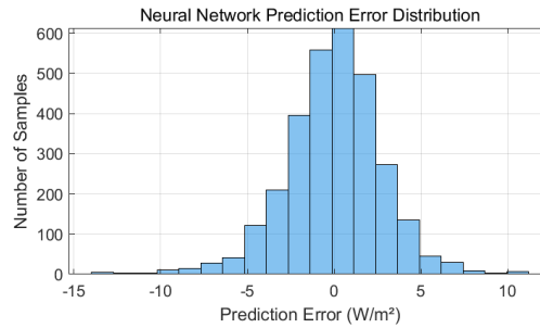
FIGURE 4. Neural network prediction error (photo/picture credit: original).
