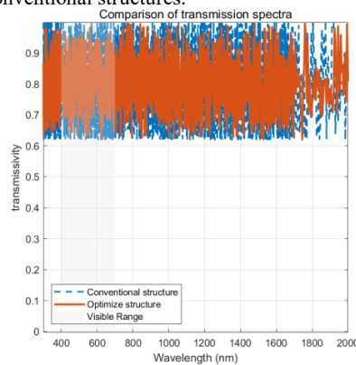
FIGURE 6. Comparison of transmission spectra (photo/picture credit: original).
