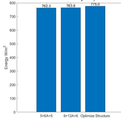
FIGURE 2. Comparison of energy transmittance of three thickness structures (Photo/Picture Credit: Original).
