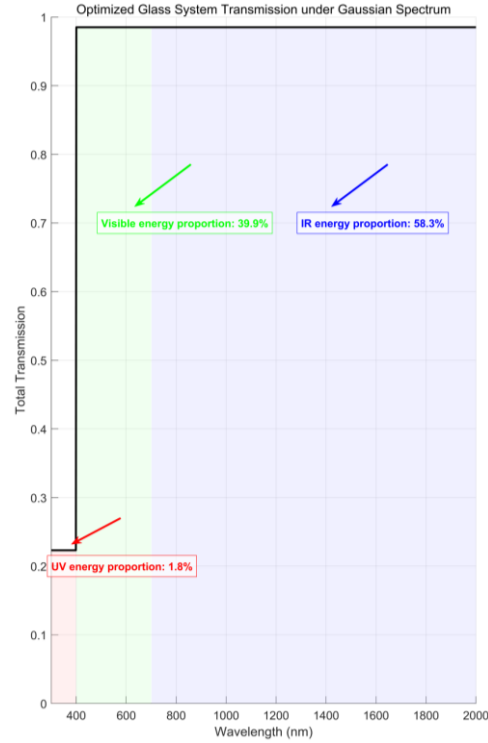
FIGURE 2. Total transmission and energy distribution by spectral band under Gaussian spectrum input (photo/picture credit: original).
