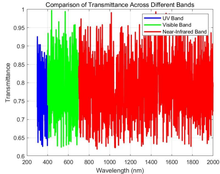
FIGURE 4. Comparison curves of transmittance in different bands (photo/picture credit: original).
