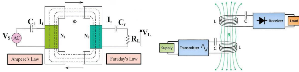
Figure 1. Wireless charging system architecture
