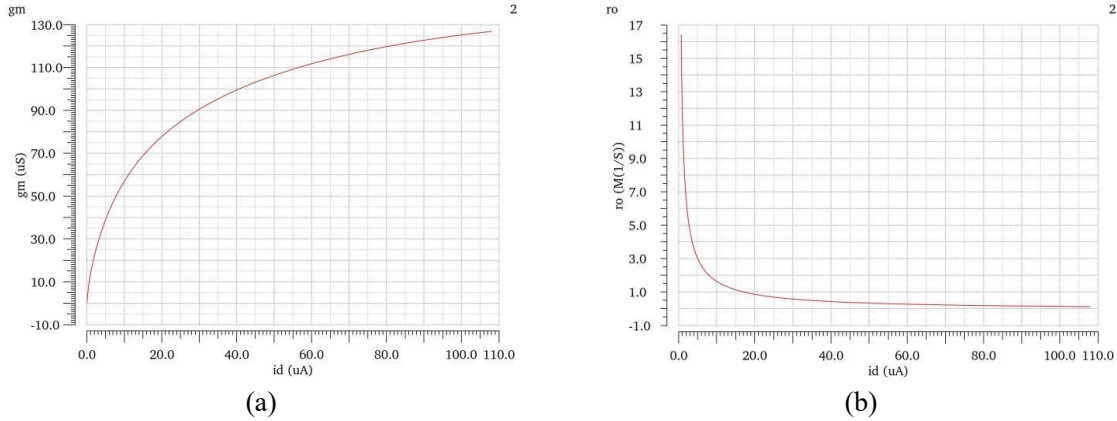
FIGURE 2. The result of PMOS simulation, (a) the relationship curves of g_m and I_d ; (b) the relationship curves of r_o and I_d . (Picture credit: Original)
