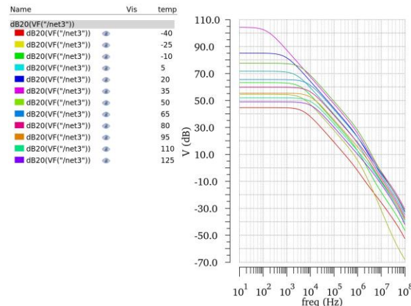
FIGURE 12. AC analysis at different temperatures.(Picture credit: Original)
