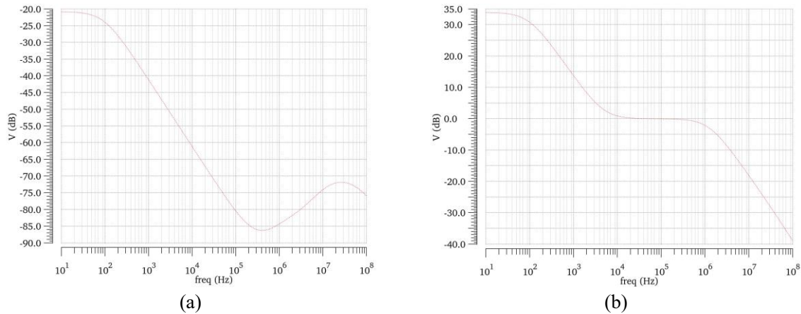
FIGURE 11. a) Common model input gain AC analysis, b) power source small signal gain AC analysis.(Picture credit: Original)
