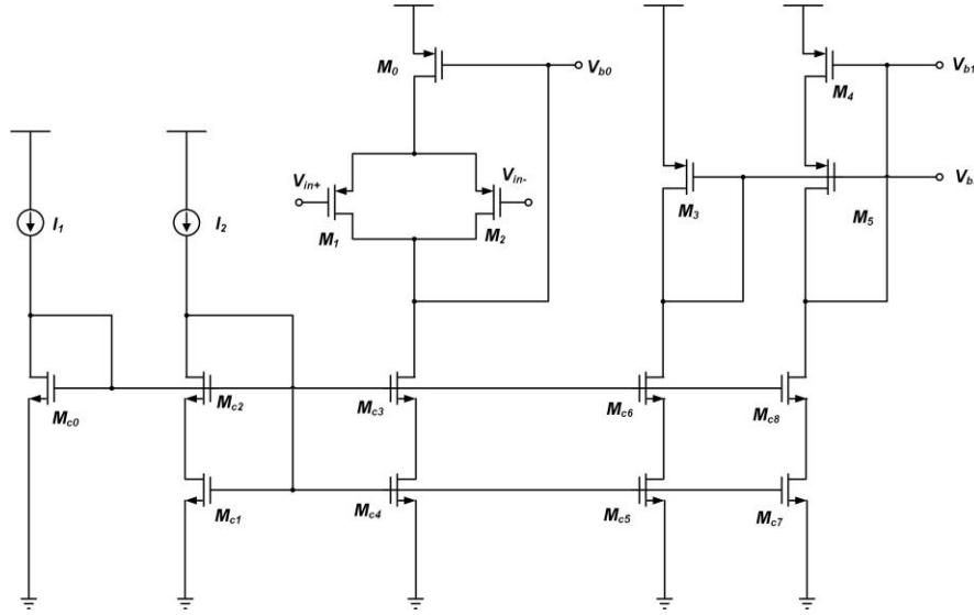
FIGURE 7. the structure of bias circuits.(Picture credit: Original)
