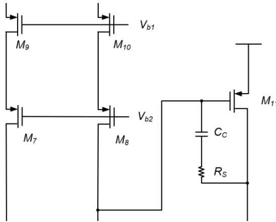
FIGURE 8. the structure of RC compensation(Picture credit: Original)
