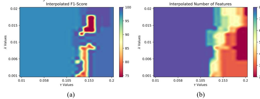
FIGURE 7. (a) Interpolated F1-Score for \lambda Values vs. \tau Values (b) Interpolated Number of Features for \lambda Values vs. \tau Values (Picture credit: Original).
