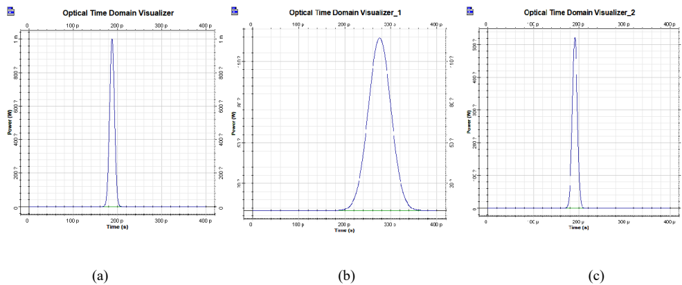
FIGURE 2. (a) The Initial Signal; (b) The Signal after passing through the Single-mode Fiber; (c) The Signal after passing through the DCF
