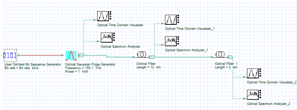
FIGURE 1. Dispersion Compensated Fiber Optic System
