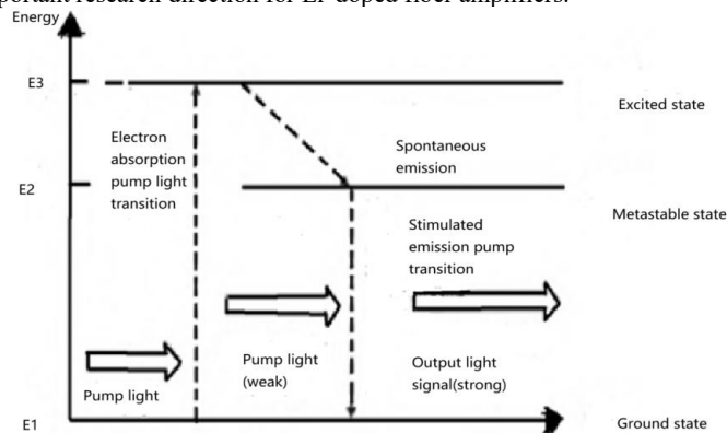
Figure 2. An erbium-doped fiber amplifier's pumping mechanism
