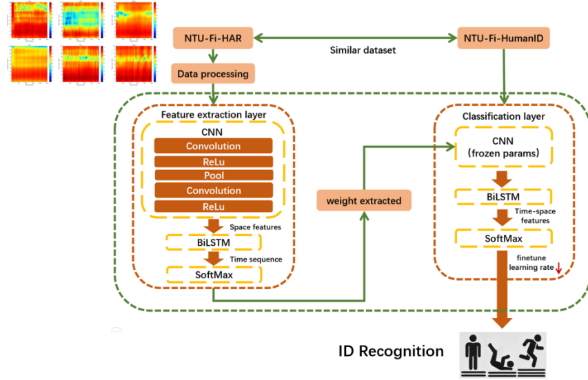
FIGURE 1. CNN-BiLSTM Transfer Learning Architecture (Photocredit : Original)
