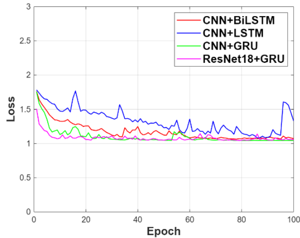
FIGURE 7. Pre-training loss for bimodal models (Photocredit : Original)
