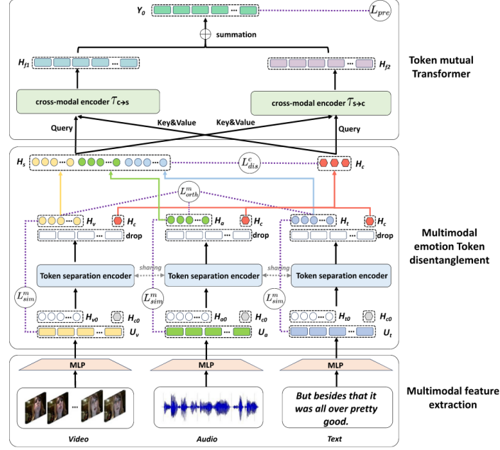
FIGURE 2. TMT framework [4].
