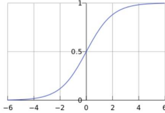
FIGURE 1. Logistic regression
