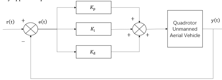
FIGURE 1. Block diagram of pid control system principle [6]
