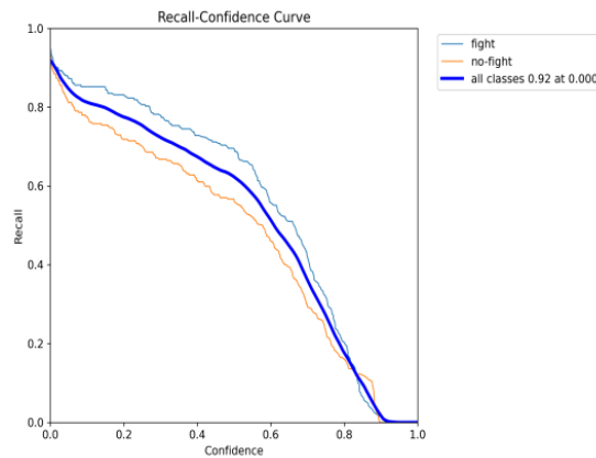
FIGURE 2. Recall-Confidence Curve
