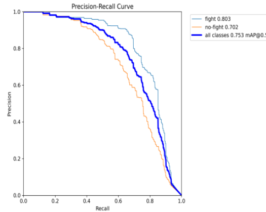
FIGURE 3. Ap Curve
