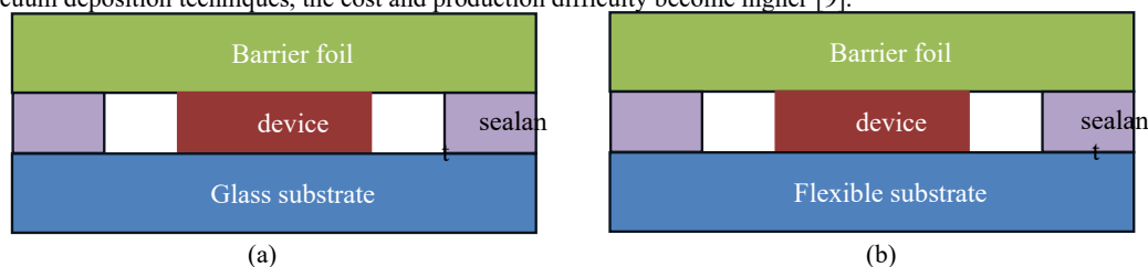
FIGURE 2. (a) The structure of the barrier foil encapsulation. (b) The structure of the thin-film encapsulation [9].
