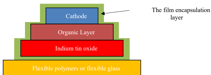
FIGURE 1. Schematic representation of thin-film encapsulation [8]
