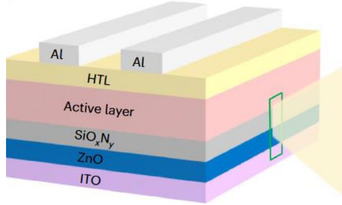
FIGURE 1. Schematic of the inverted organic solar cells [4]
