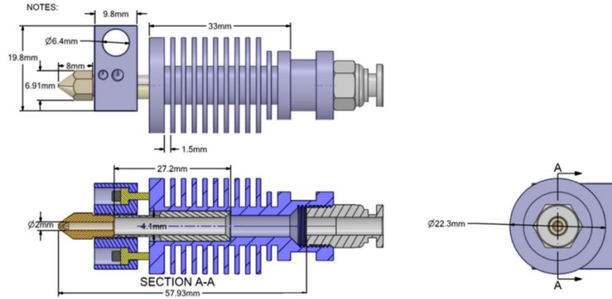
FIGURE 2. Hotend design diagram[5]
