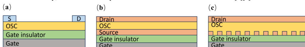
FIGURE 1. Schematic diagram of a) Traditional Planar OFET architecture (bottom gate top-contact). b) typical Vertical OFET architecture with a continuous source electrode. c) Vertical OFET with a weakly screening source electrode.
