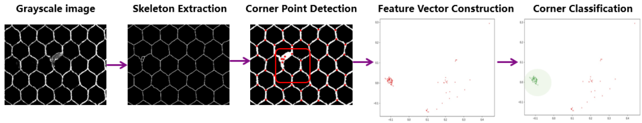
FIGURE 5. Algorithm Effect.
