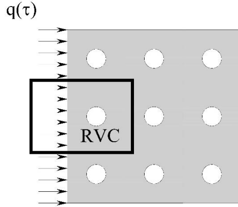
FIGURE 1. Elastic continuum with regularly distributed cylindrical voids.
