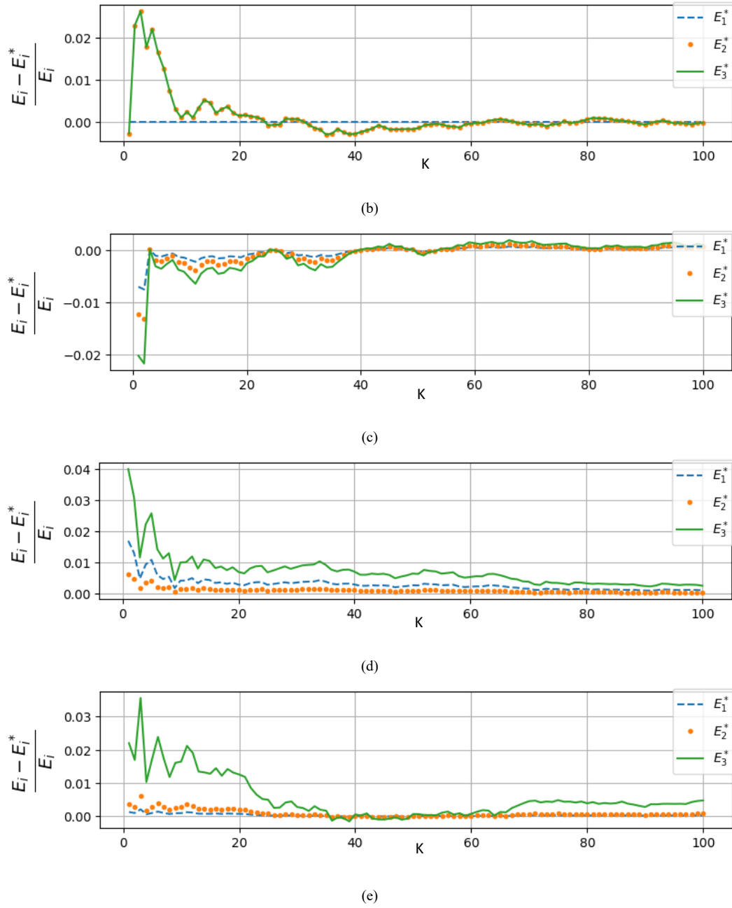
FIGURE 4. Dependence of the normalized fluctuations of estimates of Young's moduli on the number K of specimens over which the averaging was performed. The area of each face of a cubic specimen is 1\text{cm}^2 , crack radii are 1\text{mm} , the number of cracks in a specimen N = 100 . Properties of the virgin material: E_0 = 160\text{GPa} , \nu_0 = 0.3 .
