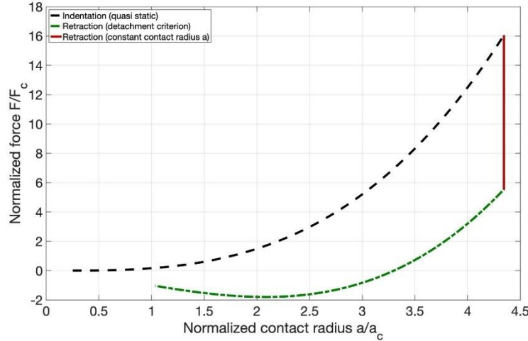
FIGURE 2. Normalized normal force vs normalized contact radius. The dashed line describes indentation (which is practically non-adhesive [5]). During detachment, the contact radius remains firstly constant (red line, corresponding to the "stick zone" [11]), followed by the JKR solution with very high effective work of adhesion (green line). Both parts of the detachment curve do not depend on the detachment velocity.
