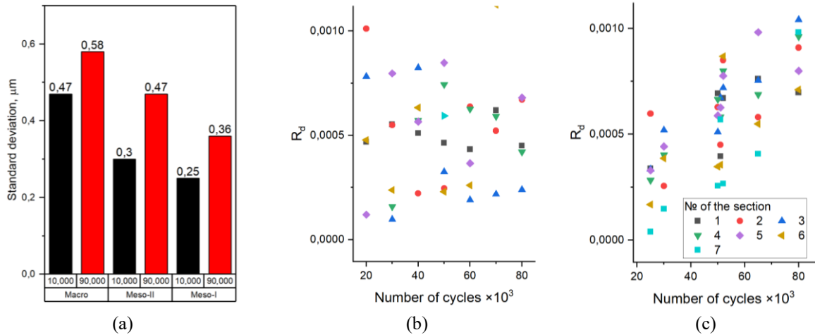
FIGURE 4. Standard deviations of the meso-I, meso-II, and macroscopic surface profile components (a), dependences of the R_d parameter on the number of cycles for the 1 st (b) and 2 nd (c) test series
