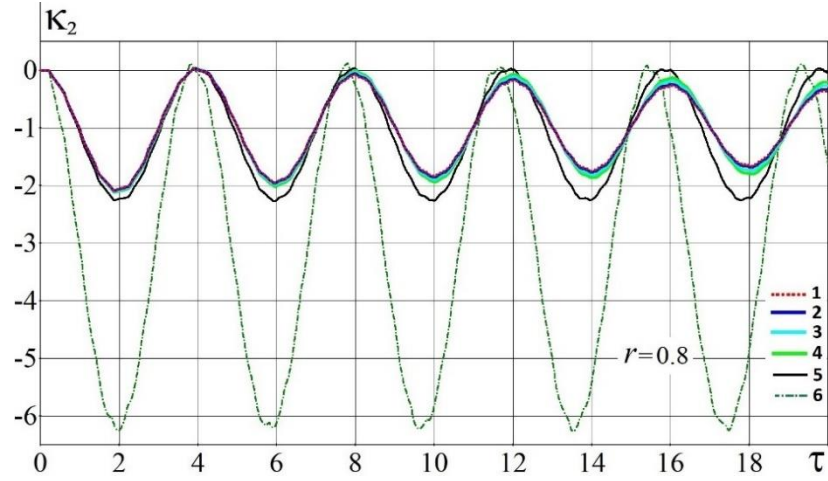
FIGURE 2. Evolution of \kappa_2 in time at the point r = r_0 = 0.8 (1 – with the regular kernel \gamma_0 ; 2 – 4 – with the singular kernels \gamma_1, \gamma_2, \gamma_3 ; 5 – for the elastic FGM; 6 – for the homogeneous elastic spherical layer)
