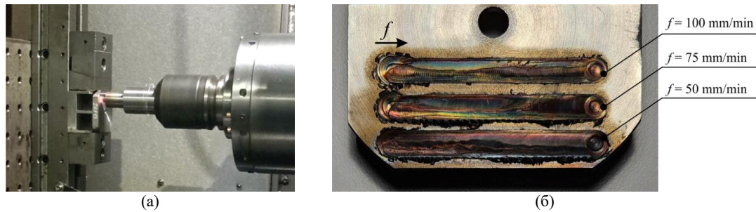
FIGURE 3. Photos of FSP at the OKUMA MA-600 processing center (a) and the friction tracks on the sample surface at feeds of 50, 75 and 100 mm/min (b)
