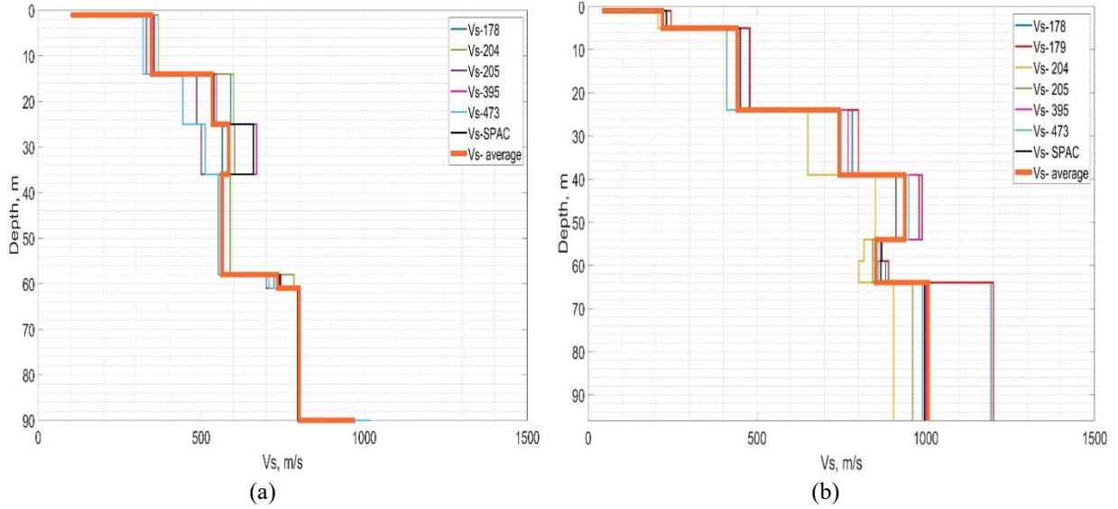
FIGURE 4. Shear wave velocity profiles obtained by the two methods – inversion of HVSR curves and MSPAC autocorrelation curves, (a) Manastirski Livadi area, (b) Loven Park area.
