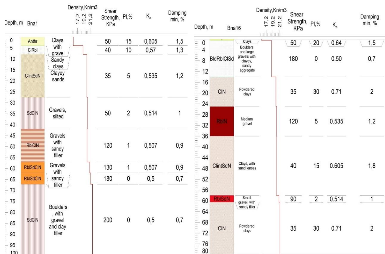
FIGURE 2. Soil stratigraphic models of boreholes Bna1 (Loven Park) and Bna16 (Manastirski Livadi). PI – Plasticity Index, K 0 – Coefficient of Earth Pressure at rest according to Darendeli [21].
