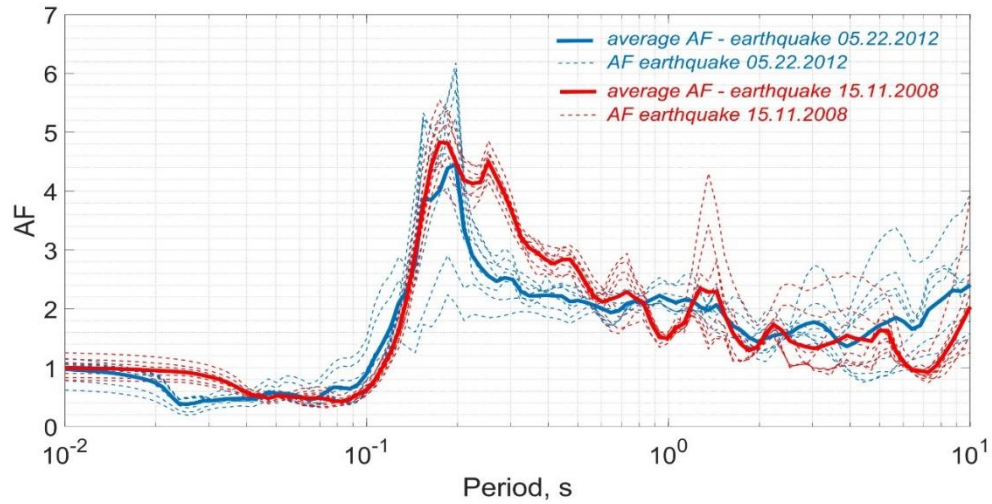
FIGURE 10. Amplification factors for the Loven park area: NL
