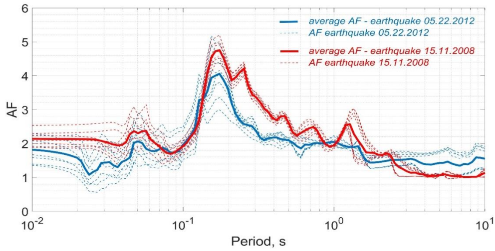
FIGURE 9. Amplification factors for the Loven park area: EQL
