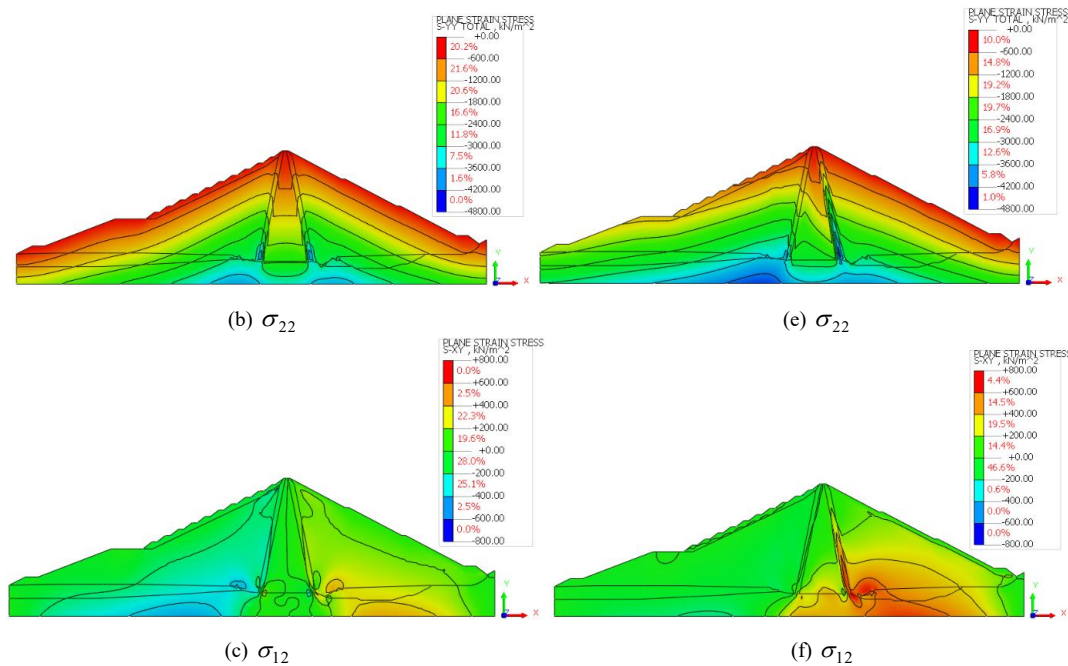
FIGURE 2. Isolines of equal distribution of stresses \sigma_{11} (horizontal, a–d), \sigma_{22} (vertical, b–e), and \sigma_{12} (shear, c–f) within the Tupalang earth-fill dam under fully impounded conditions. (a, b, c) — stress distribution resulting from self-weight and hydrostatic pressure; (d, e, f) — stress distribution resulting from self-weight, hydrostatic pressure, and seepage.
