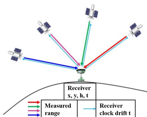
FIGURE 7. Diagram of satellite signal reception by ground devices
