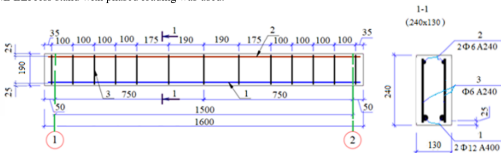
FIGURE 1. The model of beam
