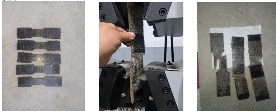
FIGURE 2. The samples of carbon and basalt tapes before and after testing
