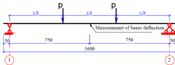
FIGURE 3. Calculation scheme for loading beams
