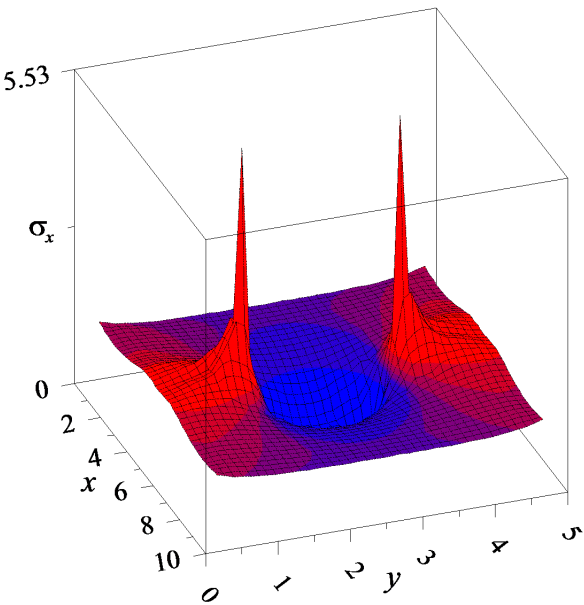
(a) Stresses along axis x
