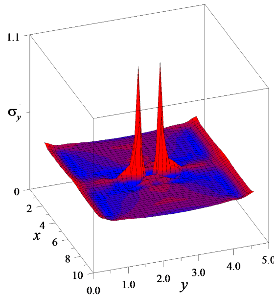
(c) Stresses along axis y
