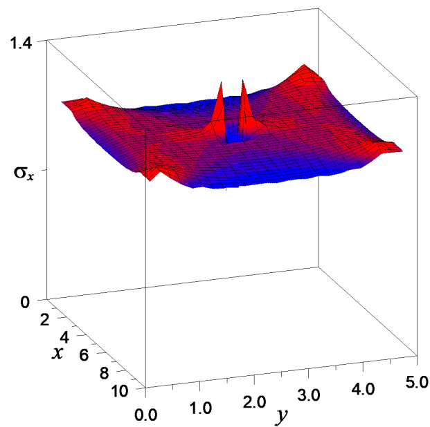
(a) Stresses along axis x
