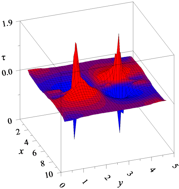
(b) Shear stresses
