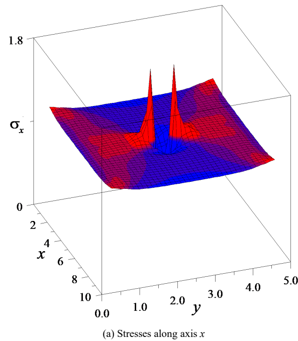
(a) Stresses along axis x
