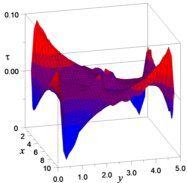
(b) Shear stresses
