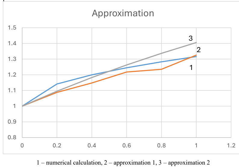
FIGURE 7. Normal stresses vs the crack length
