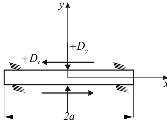
FIGURE 1. Components of a constant displacement discontinuity
