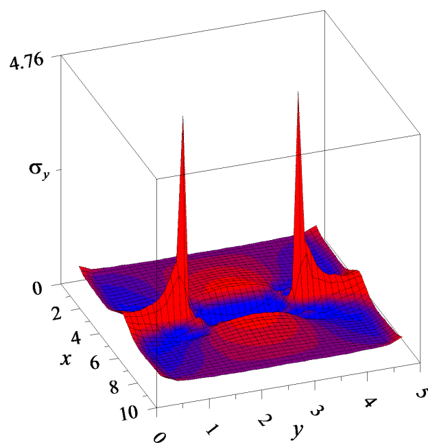
(c) Stresses along axis y
