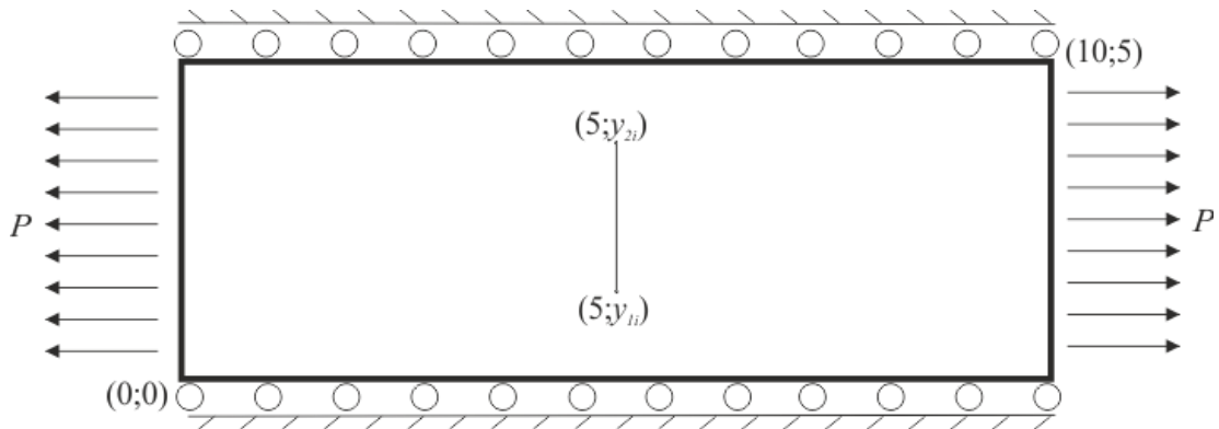
FIGURE 2. Loaded plate with initial crack
