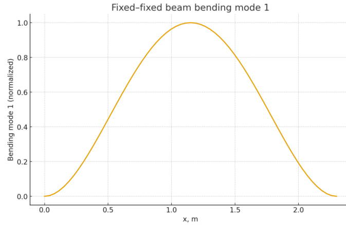
FIGURE 2. First bending mode shape (normalized amplitude)
