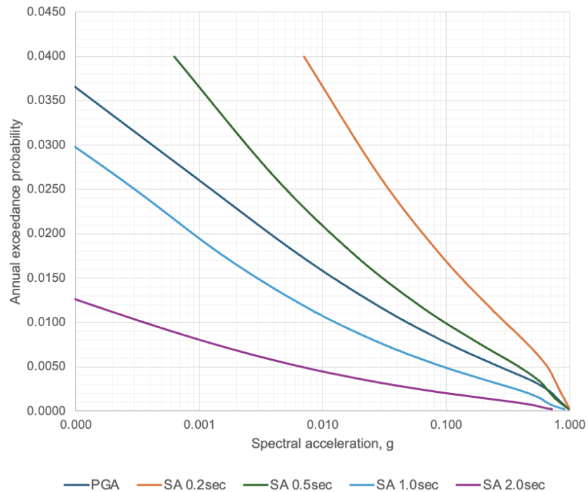
FIGURE 7. Hazard curves for selected periods of oscillation.
