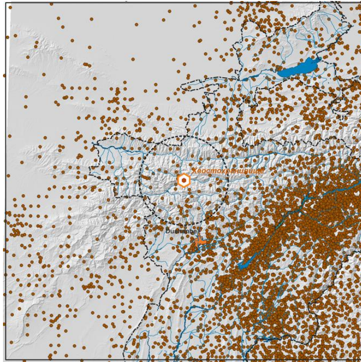
FIGURE 1. Earthquake epicenters distribution in the given area
