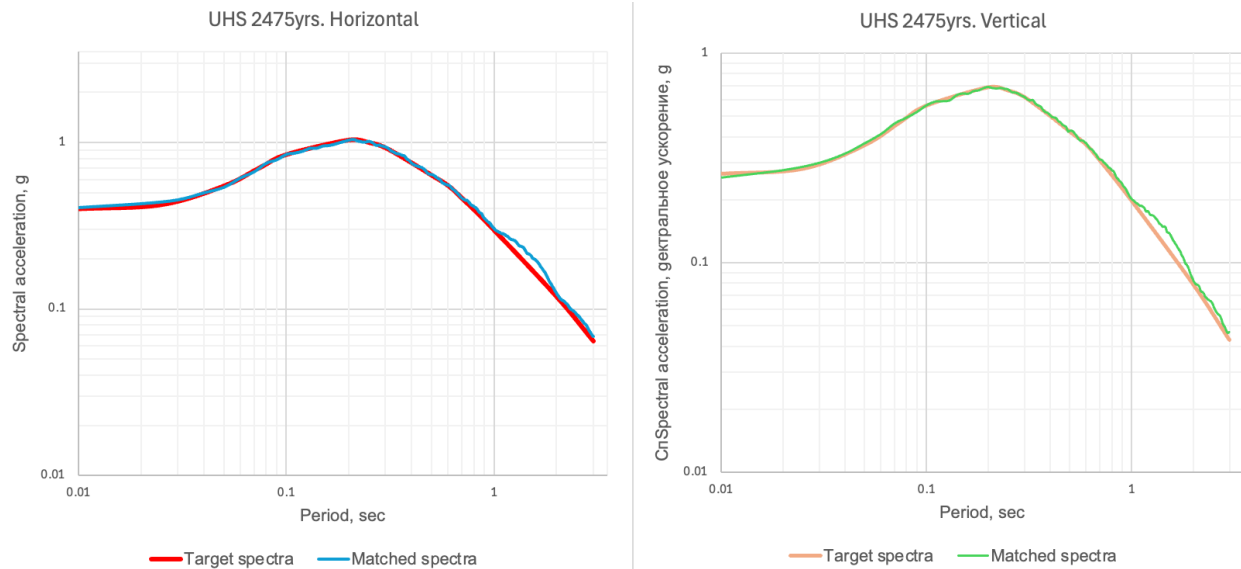
FIGURE 12. Comparison of the target spectra and spectra after spectral matching procedure
