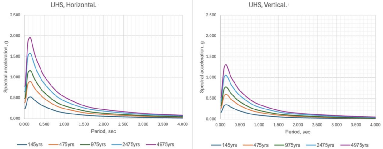
FIGURE 8. Uniform hazard spectra for given return periods
