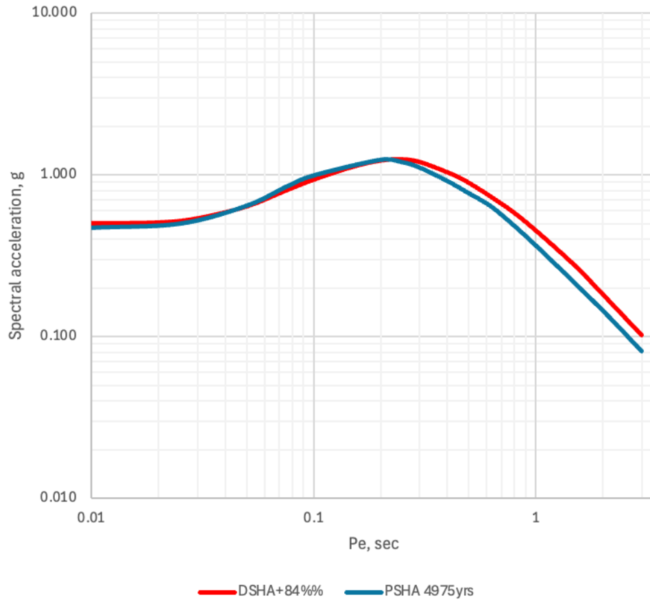
FIGURE 10. Comparing of the uniform hazard spectra from PSHA and DSHA
