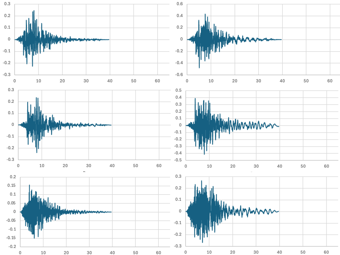
FIGURE 13. Example of results of spectral matching. Target spectra on the left, and after spectral matching are on the right
