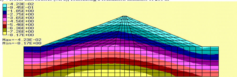
e) Shear dam stresses (MPa), considering a foundation thickness of 200 m
