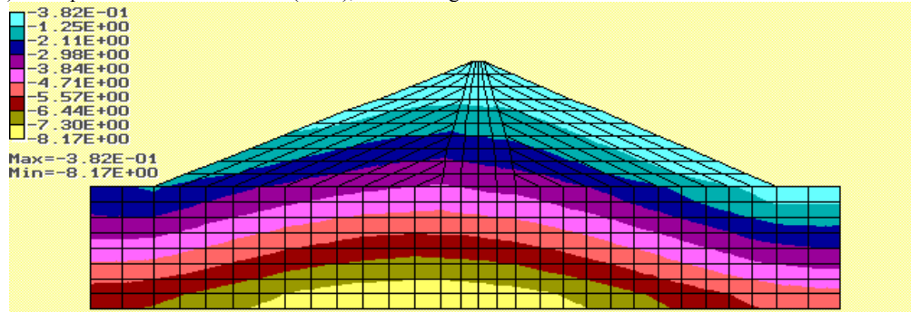
c) Dam stresses \sigma_{equ} (MPa), considering a foundation thickness of 200 m
