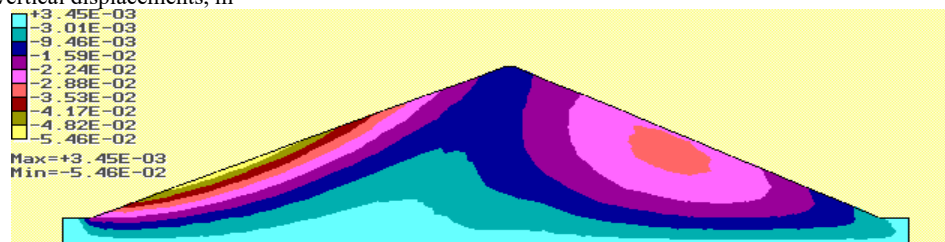
c) normal horizontal stresses \sigma_x , MPa
