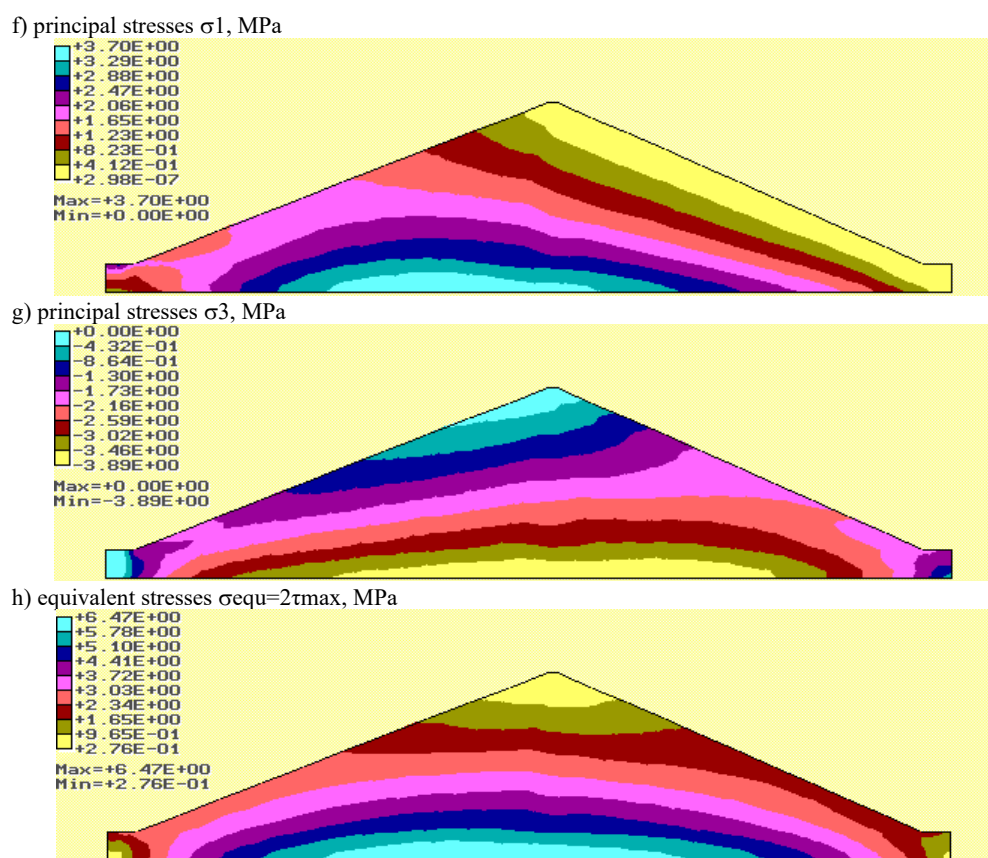
FIGURE 2. Components of the stress-strain state in a dam under seismic impact and hydrostatic pressure on the upstream slope
