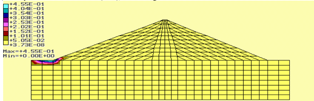
b) Principal stresses of the dam \sigma_3 (MPa), considering a foundation thickness of 200 m
