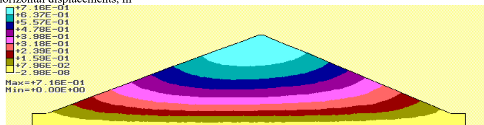
b) vertical displacements, m
