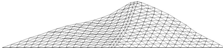
FIGURE 3. Natural modes of vibration of the dam P
