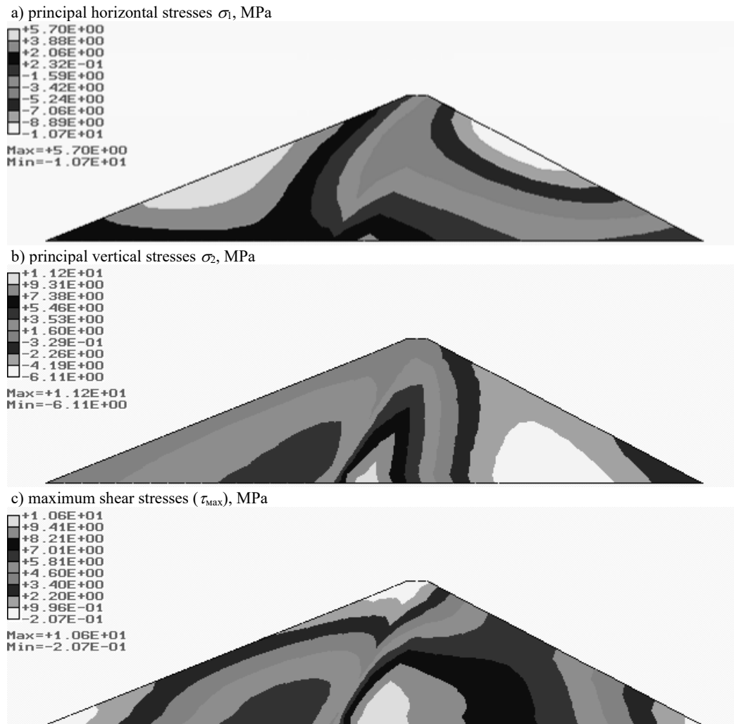
FIGURE 5. Isolines of principal stresses in the first high earth dam according to the first mode of vibrations
