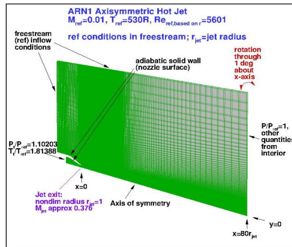
FIGURE 1. Computational grids.
