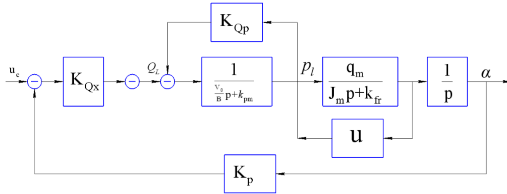
FIGURE 3. Block diagram of the optimal system
