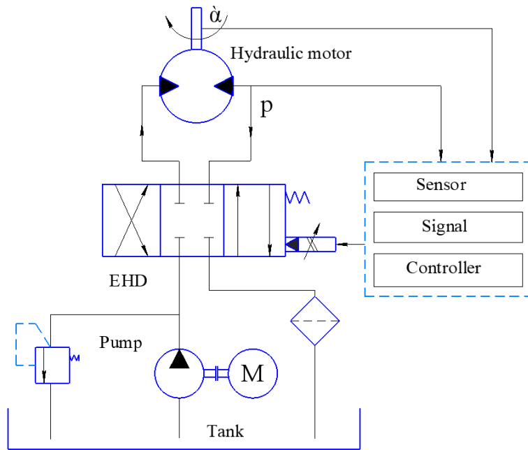
FIGURE 1. Functional diagram of the electro-hydraulic drive system
