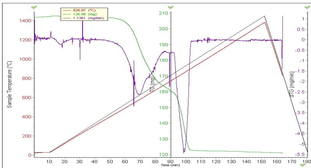
FIGURE 1. Derivatogram of phosphorite waste slurry.
