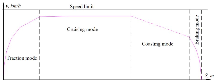
FIGURE 1. Energy-efficient control modes for long-distance train operations
