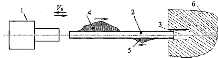
Fig.1. Schematic diagram of a technological impact system.
