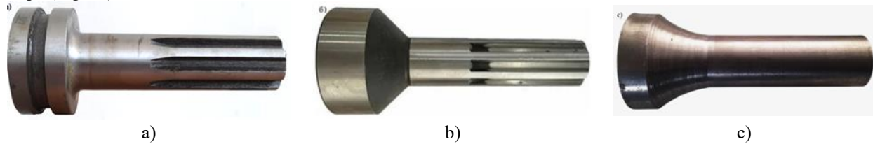
Fig. 3. General view of the piston strikers of pneumatic perforators: (a) IIII-63; (b) YT-29; (c) proposed semi-catenoid-shaped piston–striker.
