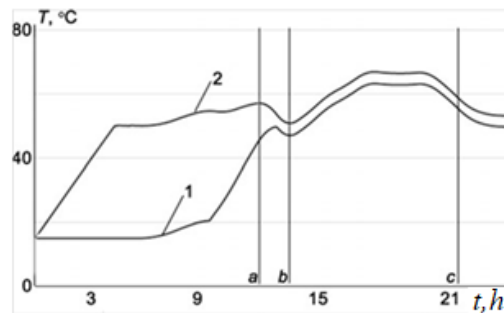
FIGURE 2. The process of changing the water temperature in the tanks:
