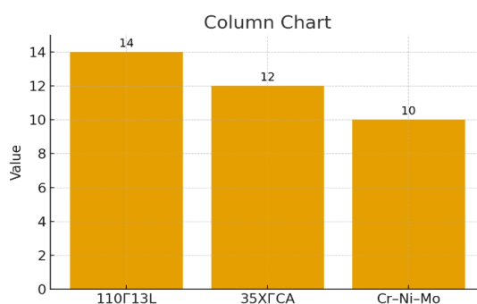
FIGURE 3. Mass loss after 8-hour abrasive cycle
