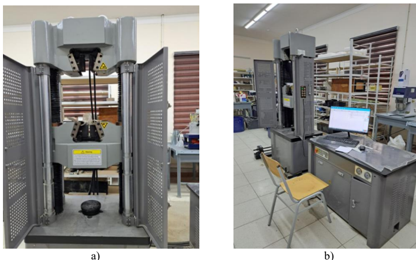
Figure 2. Alfa Test H1000 hydraulic universal testing machine; a) working section of the testing machine; b) general view of the testing machine.
