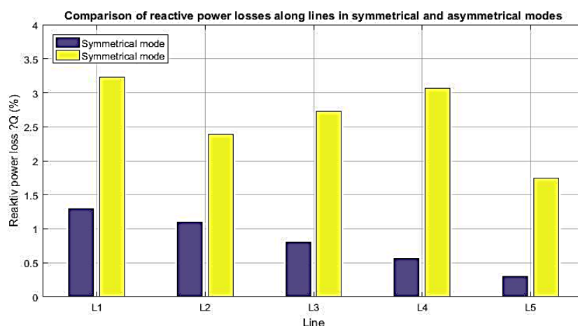
FIGURE 4. Reactive power losses in symmetric and asymmetric modes.
