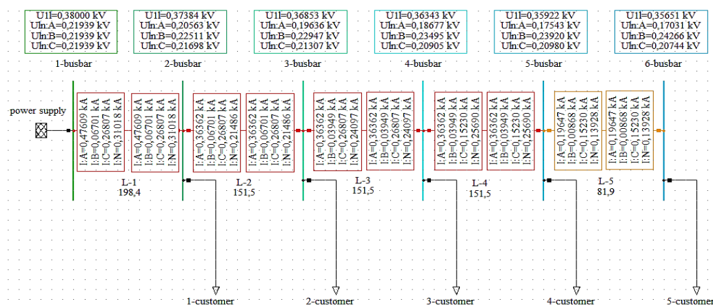
FIGURE 2. Asymmetrical diagram of a 0.38 kV network.
