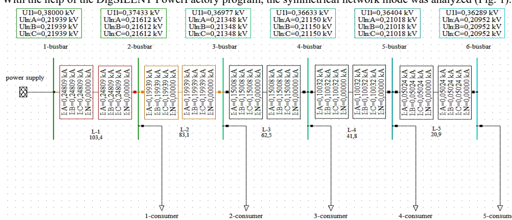
FIGURE 1. Symmetrical diagram of a 0.38 kV network.
