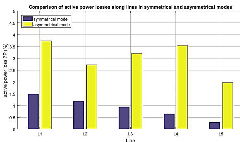
FIGURE 3. Active power losses in symmetric and asymmetric modes.
