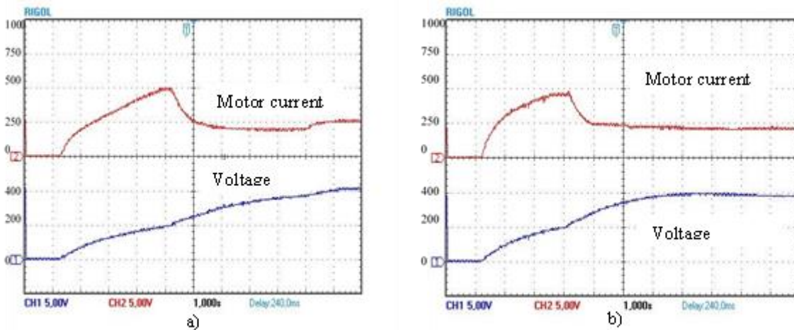
FIGURE 5. Waveforms of motor current and motor voltage with linear voltage intensity sensor (a) and S-shaped voltage intensity sensor (b).
