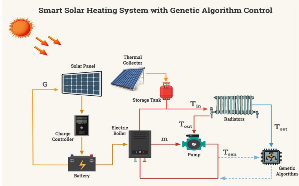
FIGURE 1. Energy-efficient heating system
