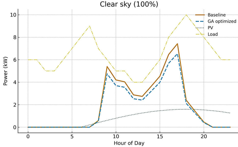
FIGURE 4. Hourly profiles of load, PV generation, and grid consumption under clear-sky conditions (100% solar irradiance).
