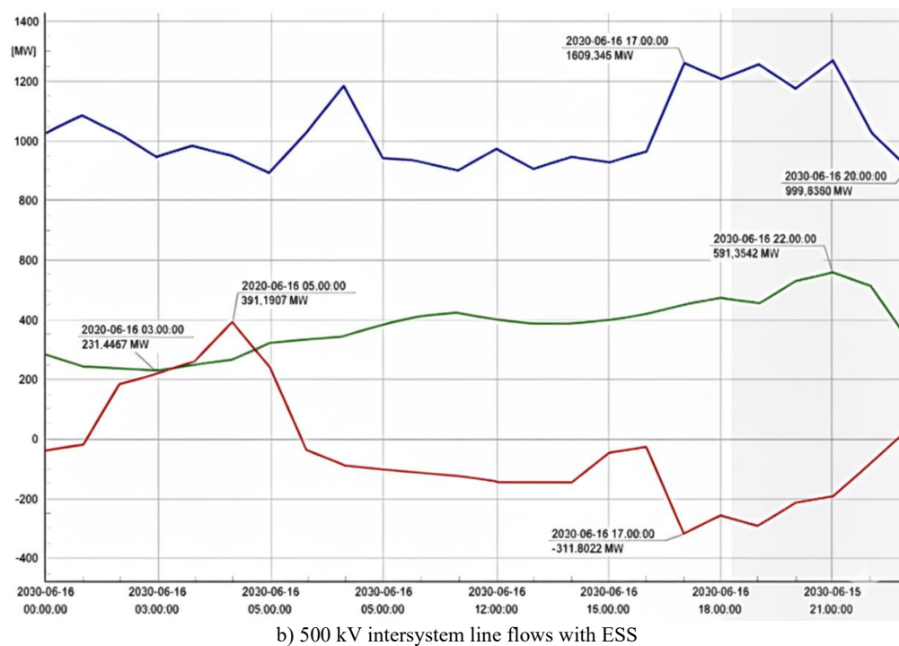
FIGURE 2. 500 kV intersystem line flows without ESS portfolio and with ESS portfolio for a typical week
