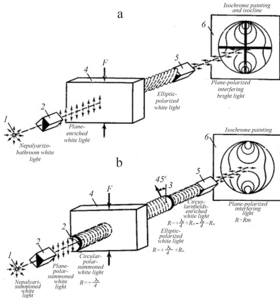
FIGURE 1. Optical polarization schemes for checking the stress state of transparent models: Conditional designations a - for plane polarization of light; b - for circular polarization of light; 1 - light source; 2 - polarizer; 3 - quarter of the plate; 4 - model; 5 - analyzer; 6 - screen. F - forces acting on the model; R - path difference of the rays; R_m - path difference of rays arising in the model; \lambda - wavelength of light.
