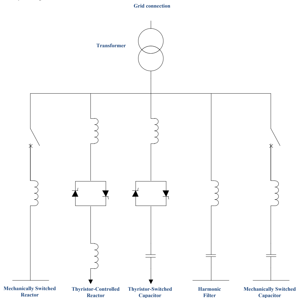
Figure 1. Single-line diagram of a static thyristor compensator
