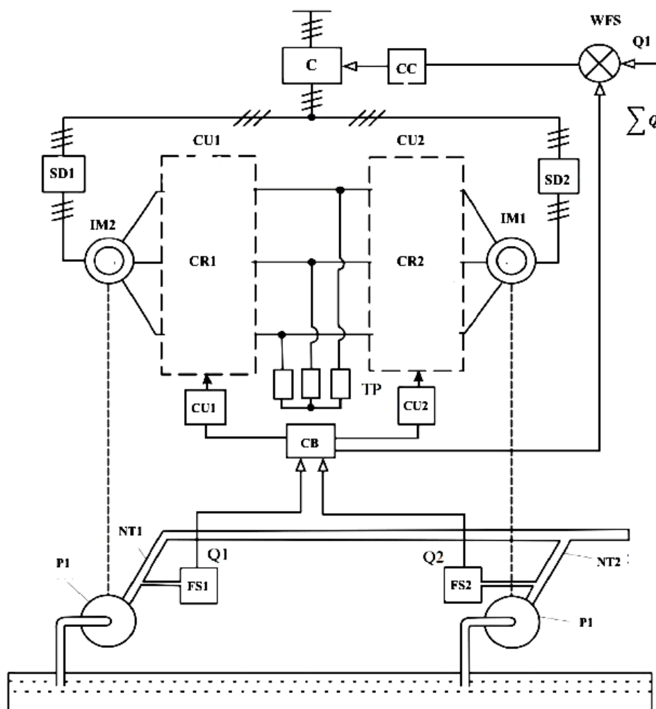
FIGURE 1. Schematic diagram of the pumping station control method using a working electrical shaft (WES) with parametric control.
