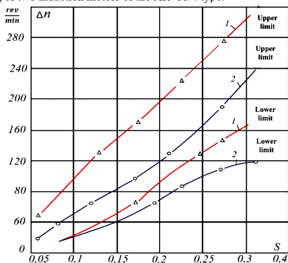
FIGURE 6. Experimental characteristics \Delta n = f(s) .
