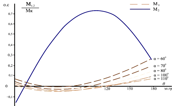
FIGURE 5. The dependences M_{1,2}/M_K = f(\theta) ПЭБ for the WES with thyristor commutators in the three phases of the rotor circuit of the less heavily loaded motor, for the case M_{c1} < M_{c2} are presented.
