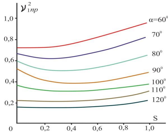
FIGURE 4. Dependencies v_1^2 = f(s)
